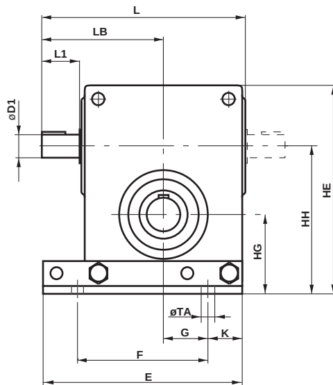
Mounting position OV, OH, OD
