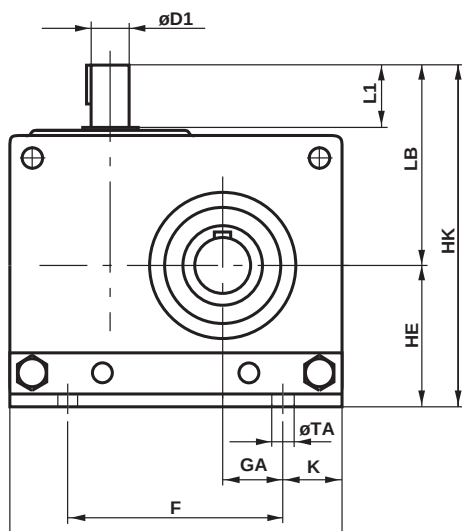
Mounting position VV, VH, VD
