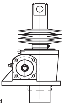
Screw jack with PVC Bellow
