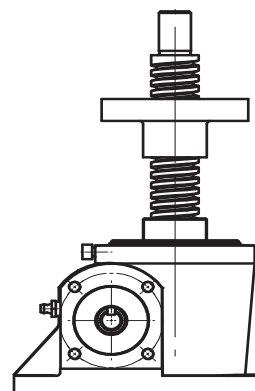
BDL Screw jack with Lifting nut
