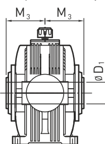
Hollow Output Shaft With Keyway - (K)
