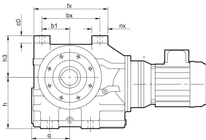
STANDARD UNIT WITH TOP MOUNTED FEET
